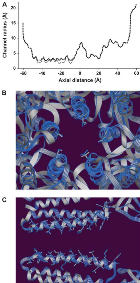
FIGURE 2 To determine the open state of the homology model, the experimental minimum pore diameter was restored by gently expanding the pore. (A) The pore radius of the closed-state homology model (dotted line) is compared to the pore radius of the expanded channel (solid line). (B) A cross-sectional view of the pre- (blue line ribbon) and postexpansion (gray solid ribbon) channel models and 2' residues (stick models) taken from the intracellular aspect. The total root-mean-squared deviation in the transmembrane region of the pore is 0.1 Å. (C) A side view of the transmembrane region of two subunits (one \alpha 1 and one \beta 2 ) of the superimposed structures. The preexpansion structure is shaded blue and the postexpansion structure is gray. Residues from the M2 domain and M2–M3 linker region are shown as stick models. In this and all subsequent figures of the receptor model, the extracellular boundary is on the right and the cytoplasmic boundary is on the left.
