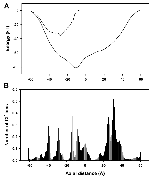
FIGURE 5 Multiion energy profile and the dwell histogram. (A) The energy well seen by a single ion (solid line) is largely reduced when seven \text{Cl}^- ions are placed in the extracellular vestibule and oval chamber. A single \text{Cl}^- ion entering the selectivity filter of the channel, with seven ions already in the extracellular vestibule, experiences an energy well 35-kT deep (dashed line). (B) To determine the regions where the resident ions reside preferentially, the channel is divided into thin sections and the average number of ions in each section during a Brownian dynamics simulation period of 0.5 \mu\text{s} is counted. The resulting dwell histogram shows many prominent peaks and troughs, representing binding sites in the channel. The histogram shows that the channel contains an average of 10.5 \text{Cl}^- ions, where 3.4 of these are located in the selectivity filter. For reference, the ring of gating Leu-9' residues is located at approximately z = -33 \text{ \AA} .
