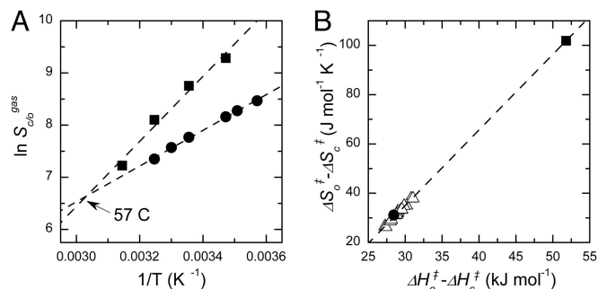
Fig. 4. The higher the CO 2 /O 2 specificity, the more it is eroded by increasing temperature. (A) Arrhenius-style plots of the specificities of the Rubiscos from spinach (●) (32) and the red alga, Galdieria partita (■) (33). (B) Positive correlation between (\Delta H_o^\ddagger - \Delta H_c^\ddagger) and (\Delta S_o^\ddagger - \Delta S_c^\ddagger) (Eq. 1) for these Rubiscos plus those from 15 C 3 higher plants (Δ) (34). To remove variation due to the differing effects of temperature on the solubilities of CO 2 and O 2 , data for S_{c/o} at various temperatures were expressed in terms of the gas-phase partial pressures of CO 2 and O 2 ( S_{c/o}^{gas} ) by dividing the reported values (which were expressed in terms of aqueous-solution concentrations) by the ratio between the aqueous solubilities of O 2 and CO 2 appropriate to the measurement temperature (41). The transformed data for each Rubisco were then fitted to Eq. 1 to obtain the estimates of (\Delta H_o^\ddagger - \Delta H_c^\ddagger) and (\Delta S_o^\ddagger - \Delta S_c^\ddagger) and their standard errors. For example, (\Delta H_o^\ddagger - \Delta H_c^\ddagger) and (\Delta S_o^\ddagger - \Delta S_c^\ddagger) were estimated to be 28.5 \pm 0.6 kJ mol -1 and 31.1 \pm 2.0 J mol -1 K -1 , respectively, for spinach Rubisco; for G. partita Rubisco, the estimates were 51.8 \pm 5.3 kJ mol -1 and 102 \pm 17 J mol -1 K -1 . The lines shown are linear regressions through all of the data.
